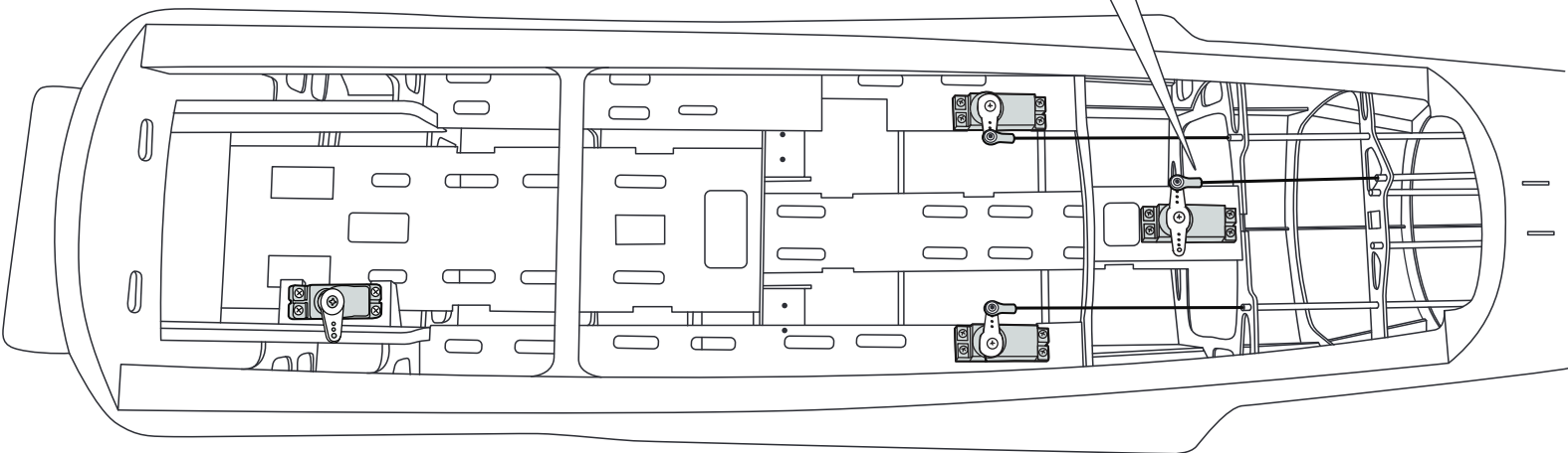
Top View
