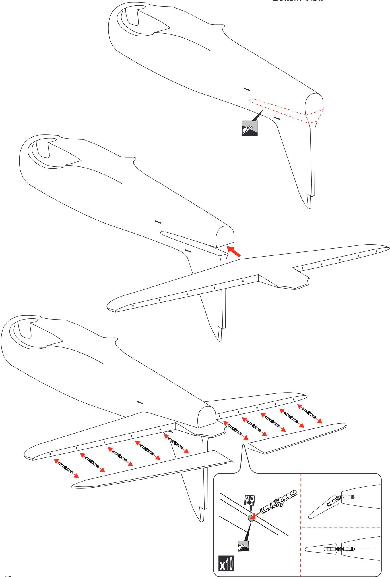
Bottom View
