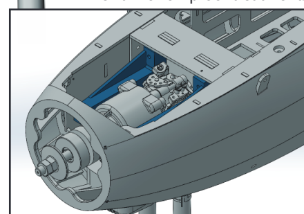
建议在防火墙上涂一层环氧树脂， 做防油处理。 It is recommended to apply a layer of epoxy resin on the firewall for oil-proof treatment.
