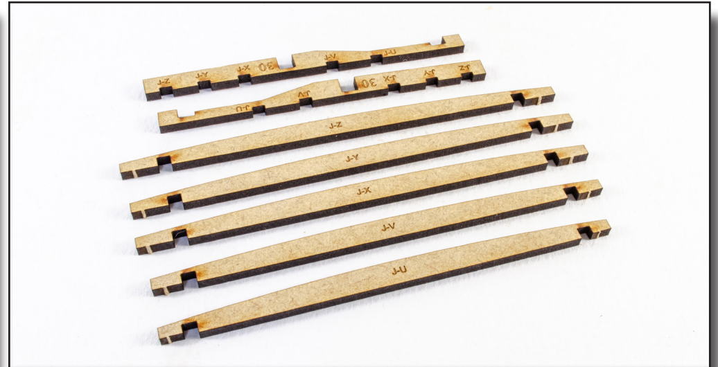
123. Before any external faces/planks are added, you'll need to get to grip with some jigs. These are designed to maintain the width between bulwarks whilst adding those external areas. From the 3mm MDF sheet, remove parts J-U, J-V, J-X, J-Y, and J-Z. Also remove parts #30. 'J' means that the parts are jigs, and these should NOT be glued to the model.
