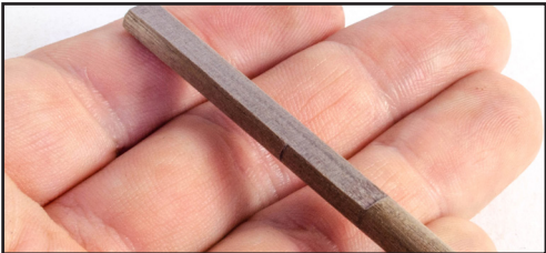
813. The mast sections will go through a number of shape changes to their cross section. Here you see the upper area of the lower section, squared-off on one side to fit the cross trees.
