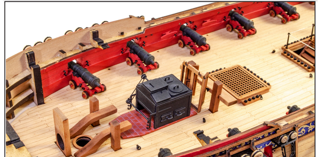
493. Now it's the turn of the cannon to be glued into position. Make sure each gun is just a little back from the bulwark and glue to the gun is central in the opening, and also at 90 degrees to the bulwarks. That of course means that the guns will have a gentle sweeping curve when fitted.
