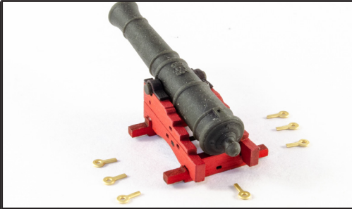
488. From the 0.4mm PE sheet, remove the Cannon Eyebolts (PE-81). You can paint these before assembly, and you will need seven per carriage.
