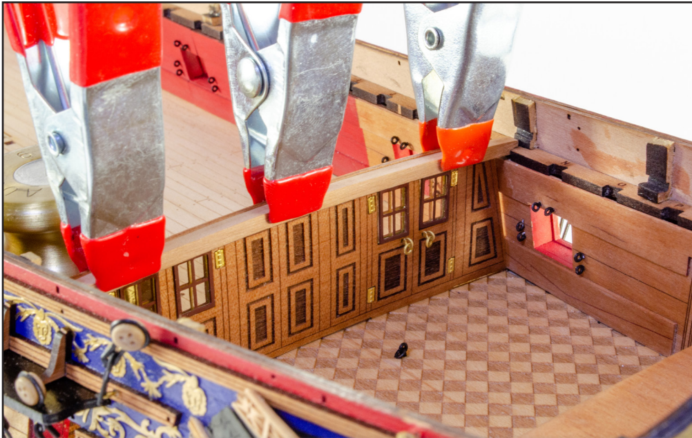
345. To help you ensure this screen is properly upright, you can glue into position Quarterdeck Beam (458M) directly behind it. The screen will sit flat up against this beam. I have also removed the laser char from the upper edges.
